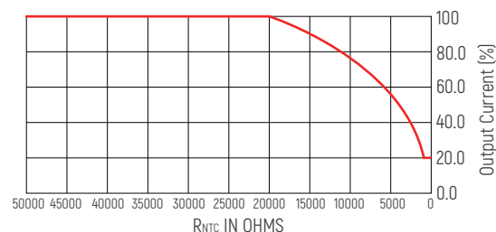
LED Thermal Protection (NTC) Characteristic
