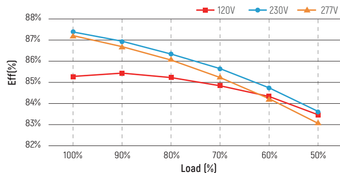
Efficiency vs Load Curve
