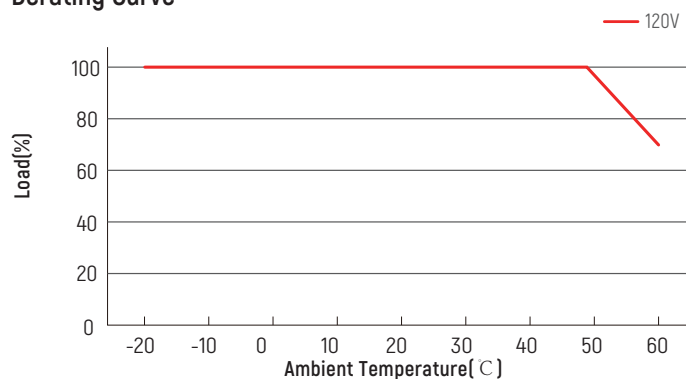
Derating Curve
