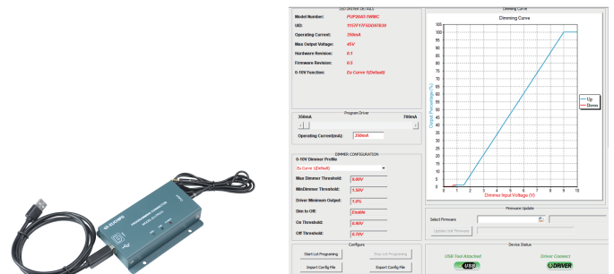
EU-PROG Programming connector
