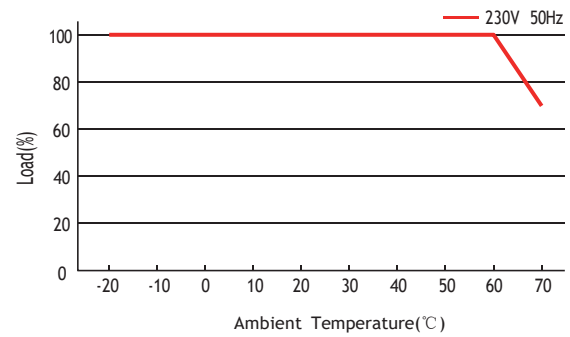
Derating Curve
