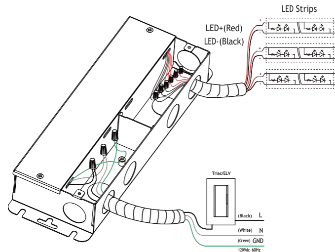
Step 3 Using Triac MLV wiring diagram
