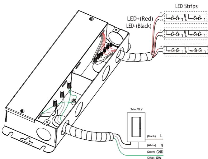
Step 4 Using Triac ELV wiring diagram
