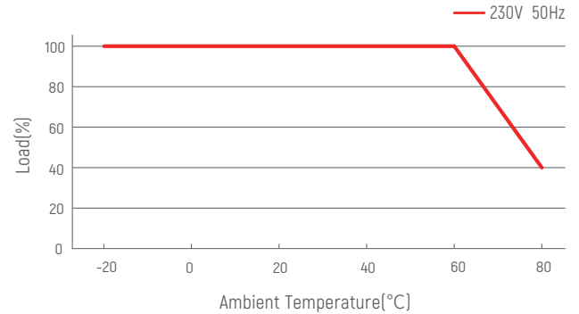
Derating Curve
