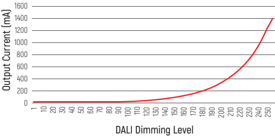
Dimming Curve
