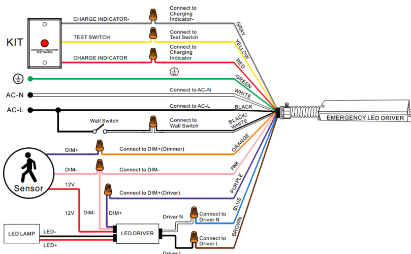
Figure C. The DC sensor and the power of the LED fixture is equal to or greater than that of the emergency LED driver.
