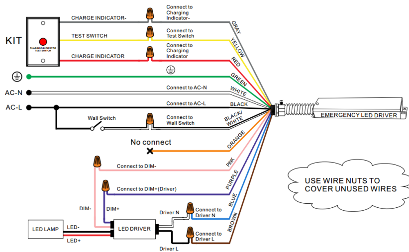
Figure A. Normal solution and the power of the LED fixture is equal to or greater than that of the emergency LED driver.
