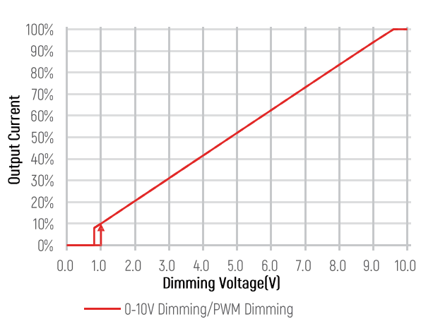
Dimming Curve
